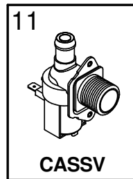
SOLENOID VALVE
