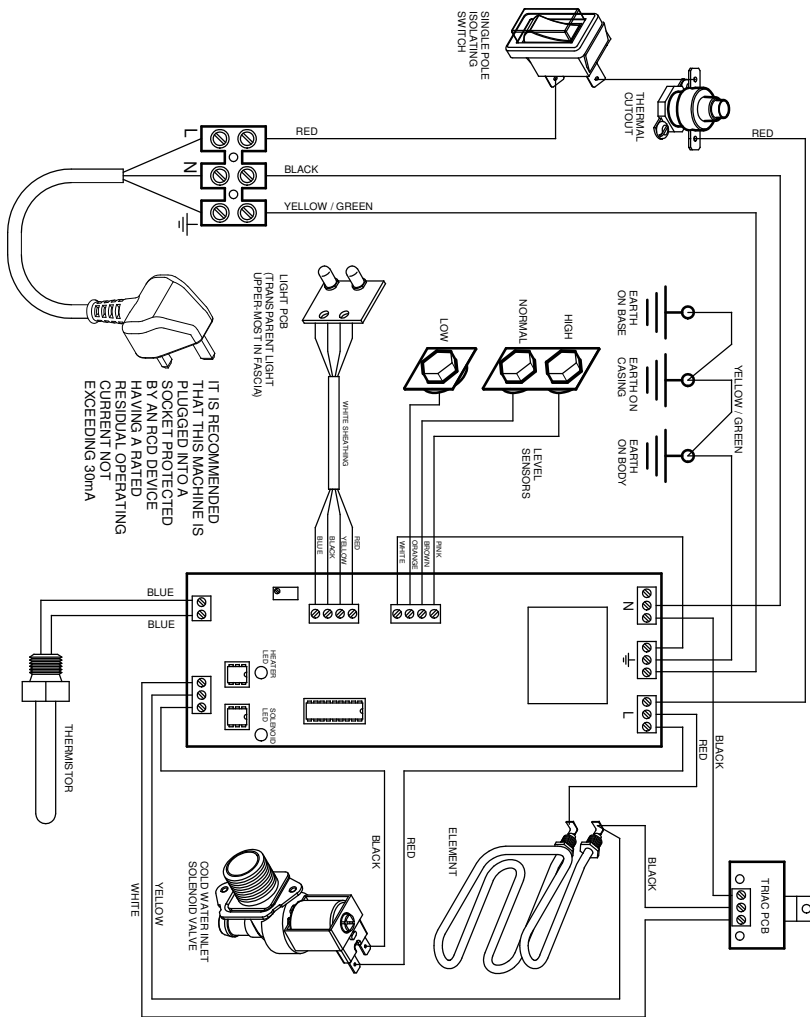
Wiring Schematic for Calomax Cascade-4 Water Boiler
