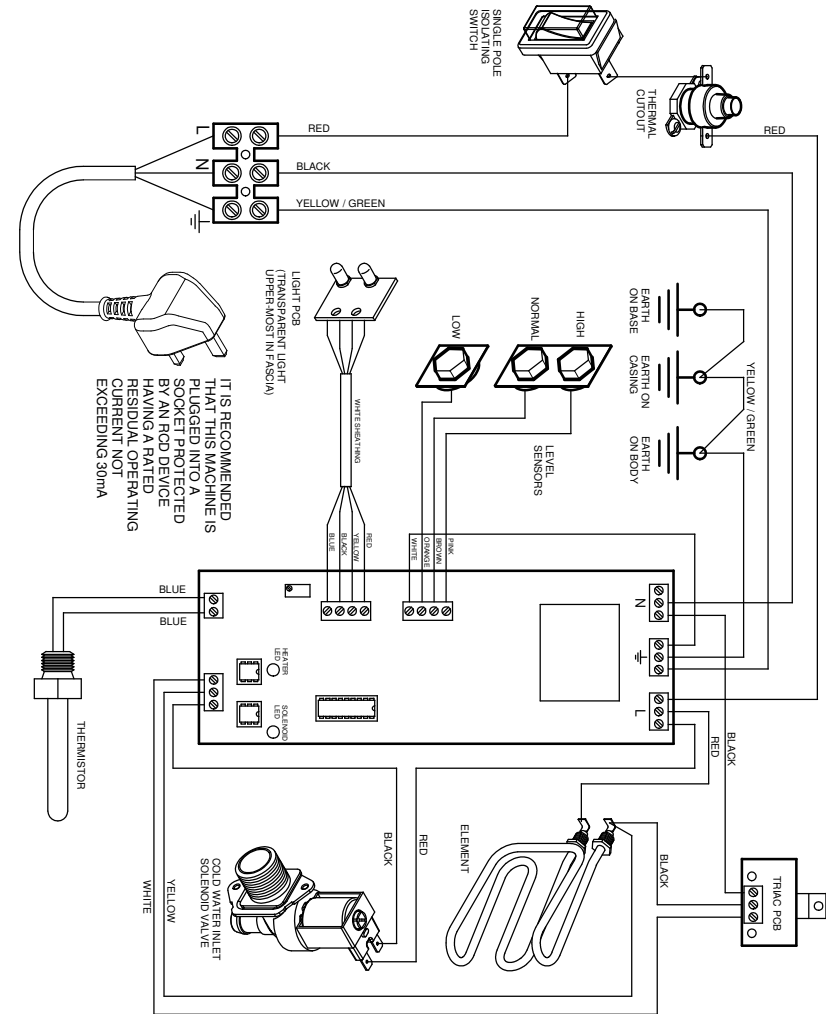
Wiring Schematic for Calomax Cascade-4 Water Boiler
